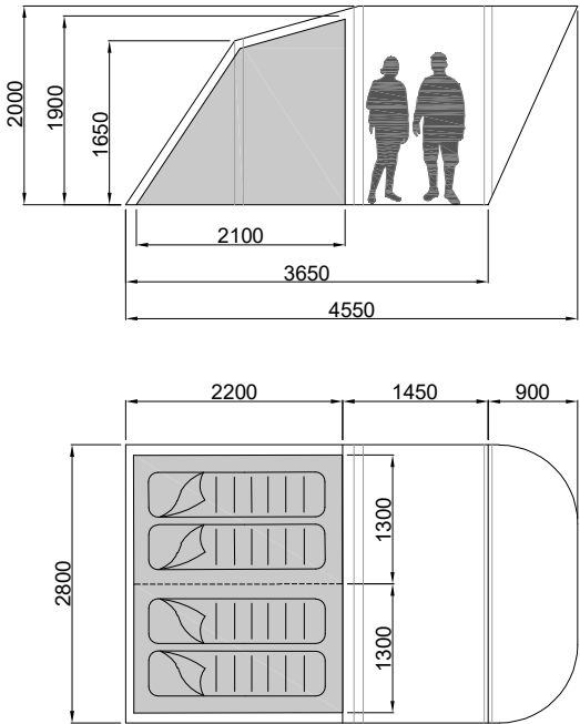
FMT Eros 4 Air
